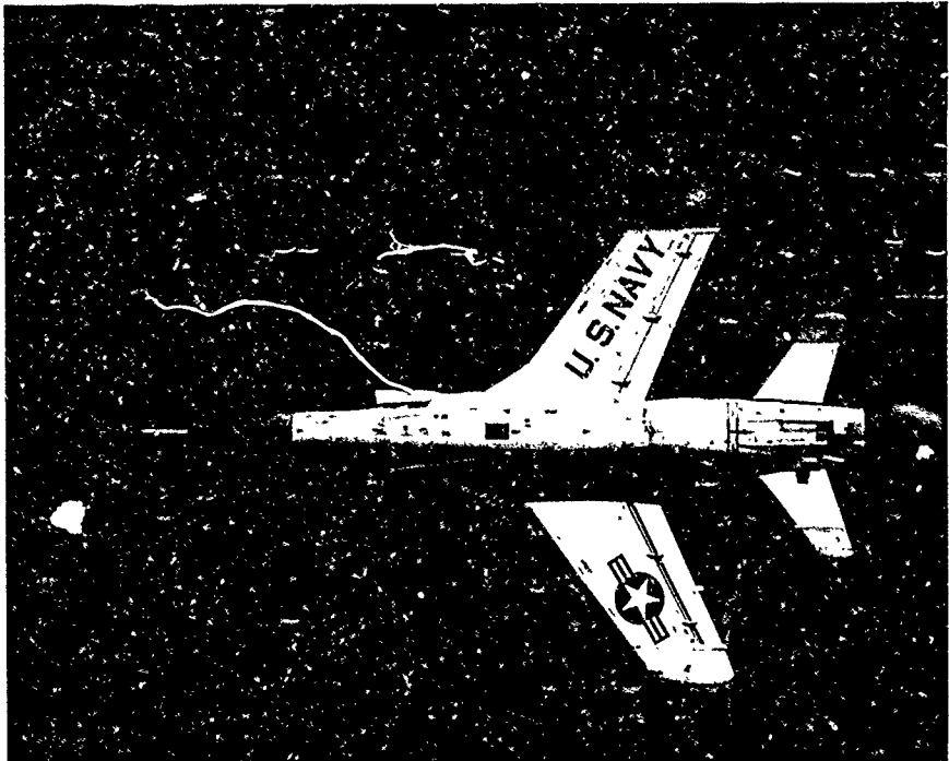
This photo taken from below the Grumman F-11 Navy fighter illustrates the way in which the area ruled fuselage was adapted to production aircraft.
