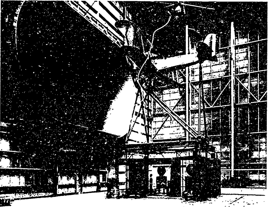
A Vought O3U set up for tests using the full scale wind tunnel at Langley, completed in 1931.
