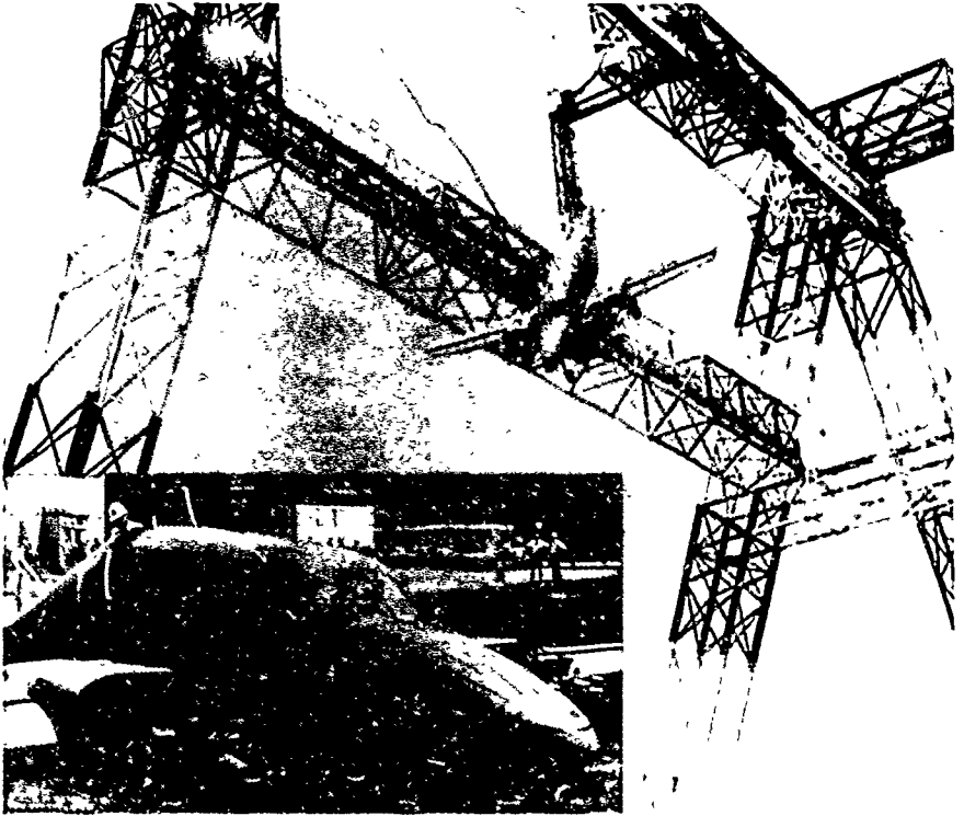
In cooperation with the Federal Aviation Administration, crash tests were aimed at developing better protection for pilots and passengers in general aviation aircraft. Crash tower and damaged plane unset.
